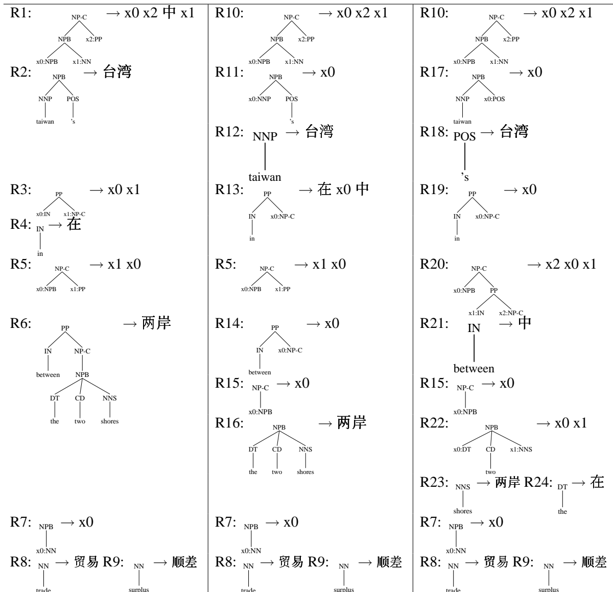
Figure 2: A (English tree, Chinese string) pair and three different sets of multilevel tree-to-string rules that can explain it; the first set is obtained from bootstrap alignments, the second from this paper's re-alignment procedure, and the third is a viable, if poor quality, alternative that is not learned.
