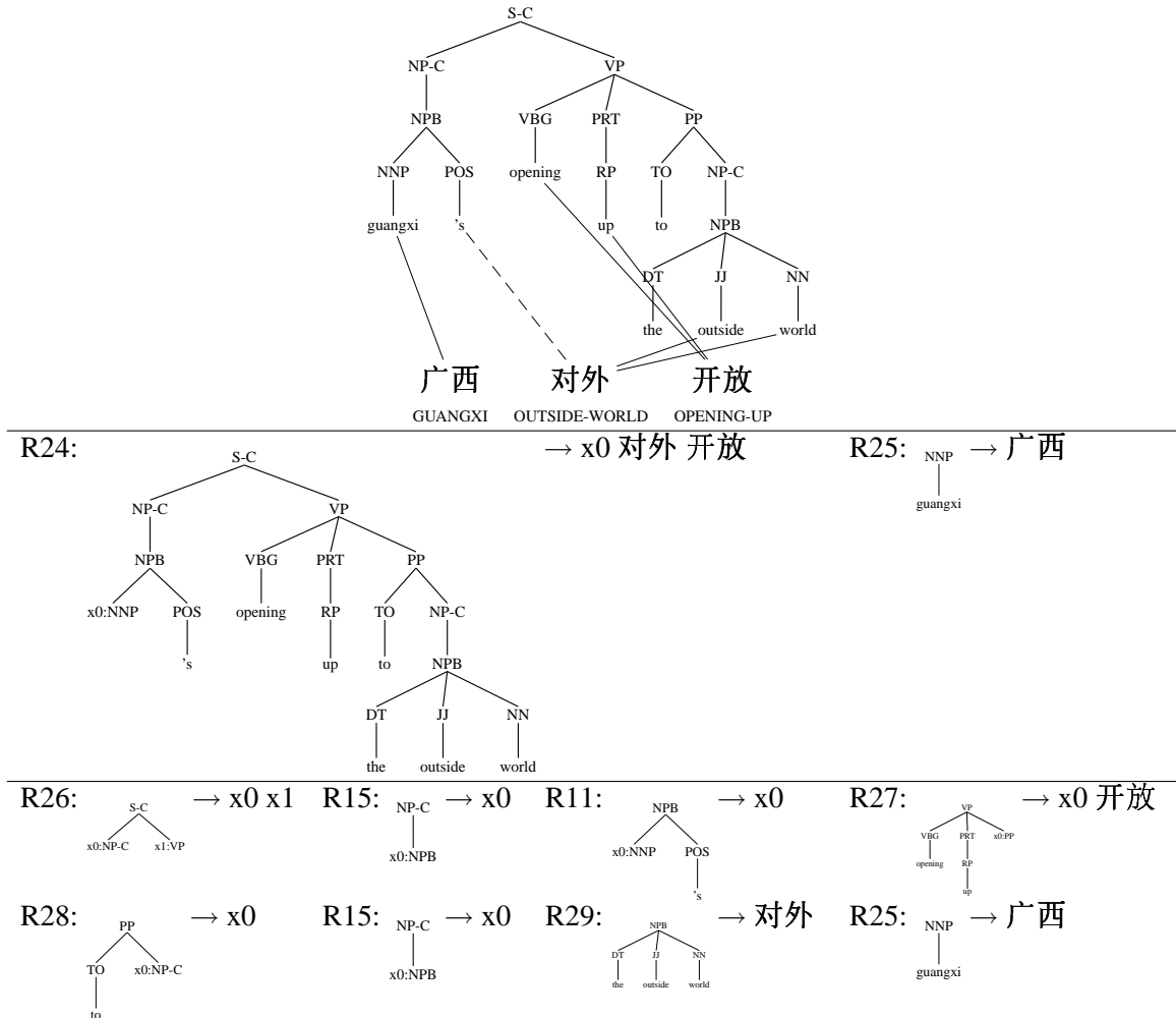
Figure 3: The impact of a bad alignment on rule extraction. Including the alignment link indicated by the dotted line in the example leads to the rule set in the second row. The re-alignment procedure described in Section 3.2 learns to prefer the rule set at bottom, which omits the bad link.
